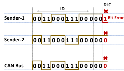
Figure 3: Producing a bit-error.
