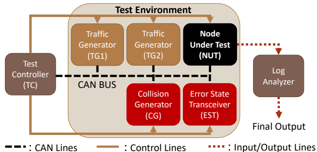
Figure 4: Architecture of CANOX.
