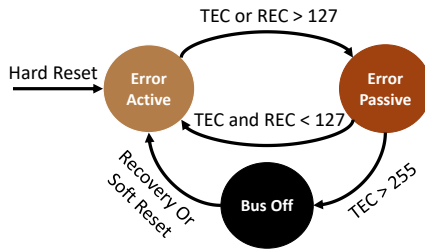
Figure 2: Error states in CAN.
