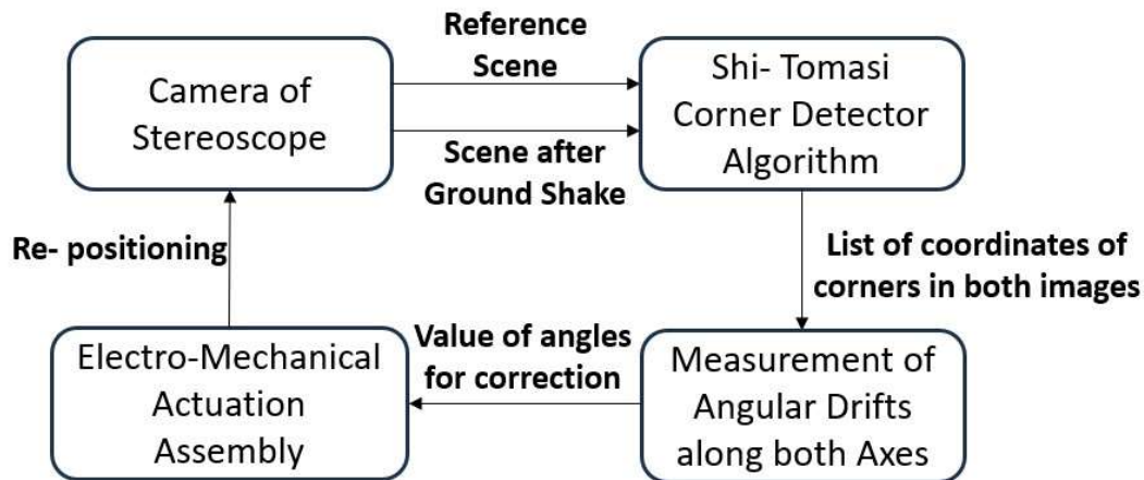
Figure 7: Offset Compensation against Ground Shake
