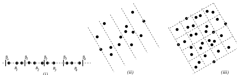
Figure 9: (i) Uniform-projection problem; (ii) two-dimensional partitioning problem.
