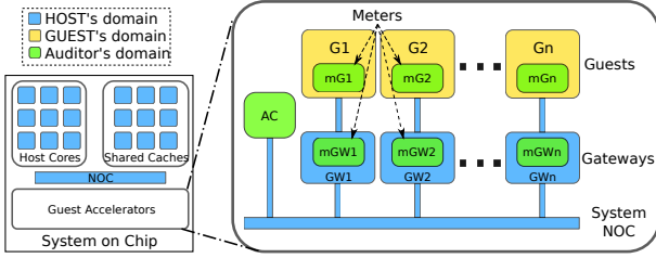
Figure 1. Hardware architecture
