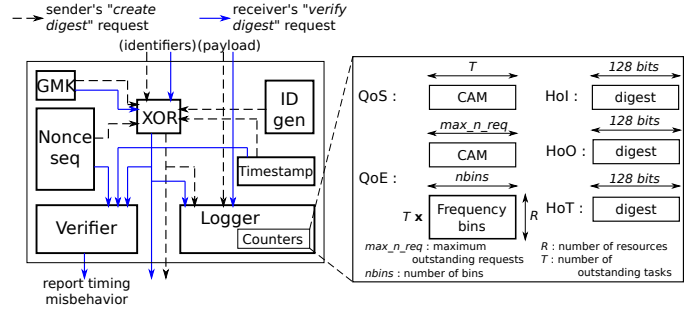
Figure 2. Structure of a meter
