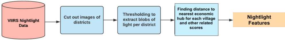
Fig. 7. Pipeline of obtaining the nightlights features.
