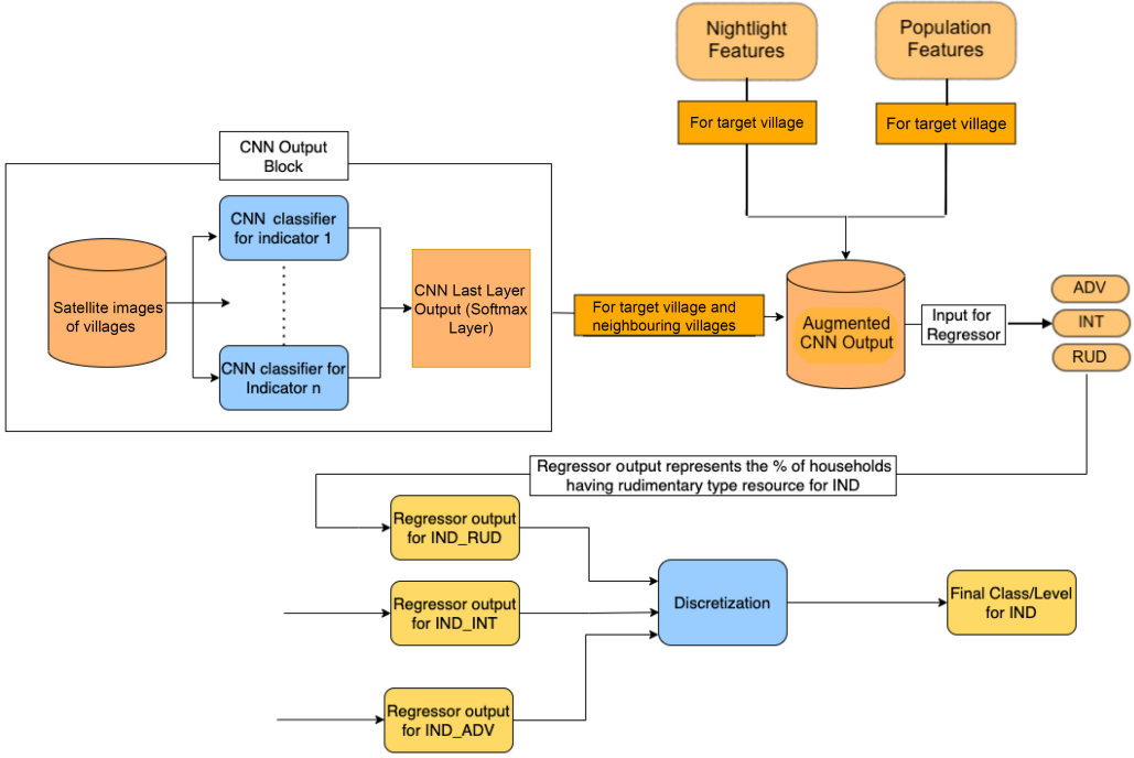
Fig. 5. Architecture-2 structure. This is a two-stage setup, with the first stage being the same as for Architecture-1, of a CNN-based model to predict the development class. The second stage takes the softmax outputs of the first stage as features; concatenates them with the same features obtained for neighboring villages, along with nightlights-based features; and uses this large set of features to learn regression models for each output. The output is then discretized to the development class (level 1, level 2, or level 3) for the village. Separate models are learned for each indicator, denoted by IND = \{BF, FC, MSW, LIT, ASSET\} .
