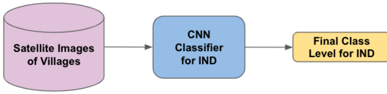
Fig. 3. Direct CNN-based classification where the model takes a village satellite image as an input and predicts the development class (level 1, level 2, or level 3) for the village. Five models were learned, one for each indicator, denoted by IND = \{BF, FC, MSW, LIT, ASSET\} .
