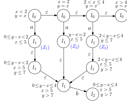
Fig. 2. Zone Graph for the TA in Figure 1
