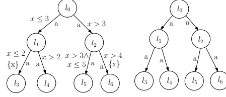
Fig. 4. The two timed automata are timed bisimilar
