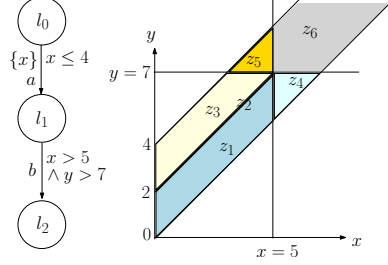
Fig. 1. A timed automaton and the zones for location l_1
