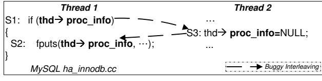
Figure 1. An atomicity violation bug from MySQL.
