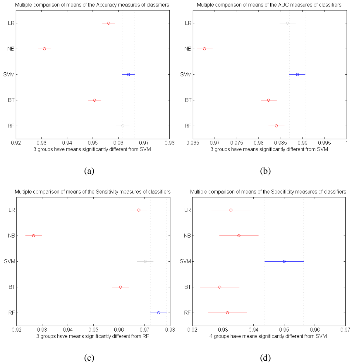
Fig. 6. Statistical comparison of the classifier performance measures using multiple comparison tests (a) Accuracy, (b) Area under ROC (AUC), (c) Sensitivity, and (d) Specificity. Note: LR, NB, SVM, BT, and RF represent Logistic Regression, Naïve Bayes, Support Vector Machine, Boosted Trees and Random Forests, respectively.
