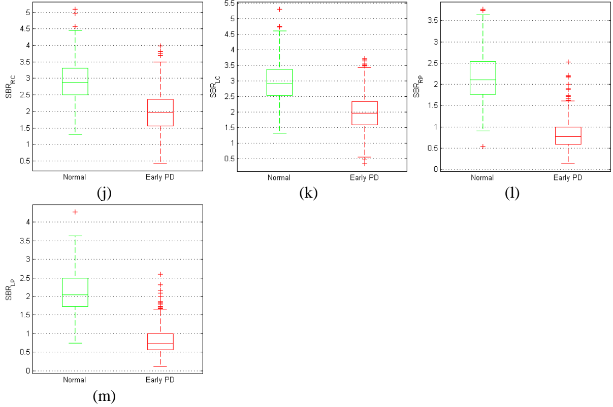
Fig. 2. Box plot of (a) RBDSQ score, (b) UPSIT score, (c) A \beta 1-42, (d) \alpha -Syn, (e) P-tau 181 , (f) T-tau, (g) T-tau/A \beta 1-42, (h) P-tau 181 /A \beta 1-42, (i) P-tau 181 /T-tau, (j) SBR RC , (k) SBR LC , (l) SBR RP , and (m) SBR LP , for normal and early PD population.
